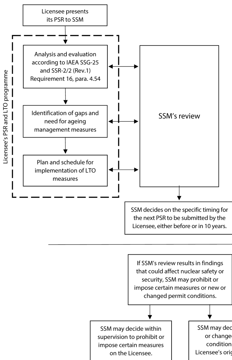
Figure 3.3. PSR and LTO review process in Sweden
